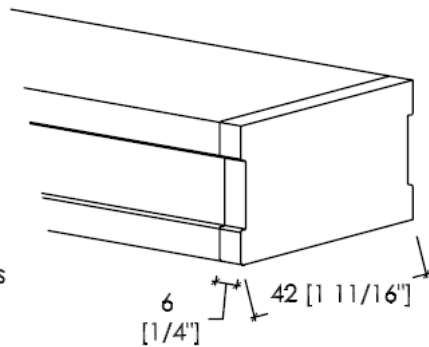
End Caps for Top Tracks (Ceiling Mounted)
