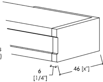
End Caps for Top Tracks (Surface/Wall Mounted)
