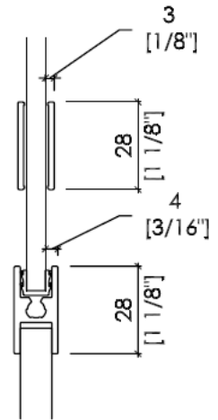
Glue-on Dividing Rail
