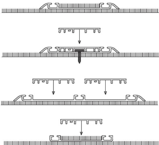
Cross section vertical: 34mm Bottom Tracks
