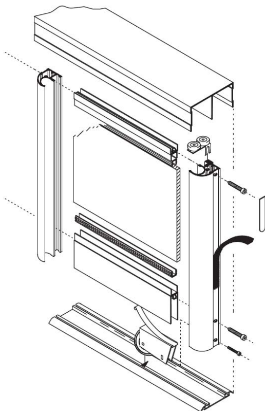
Isometric view S751
